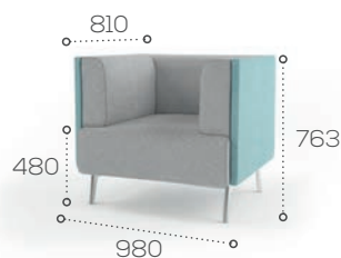
STK1 - 1 seat
